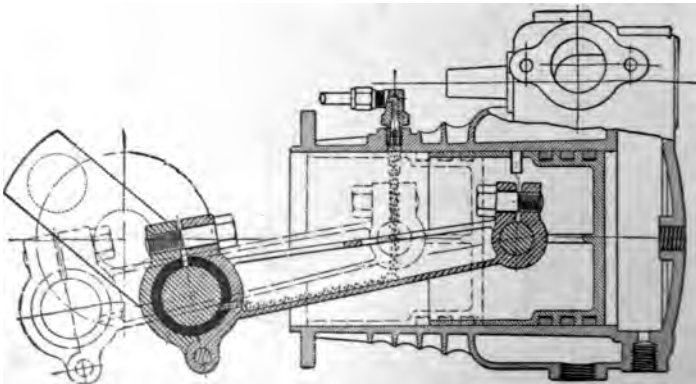
FIG. 306. —Horizontal Cylinder Oiled by Force-feed Oiler Distributor. The piston is oiled when passing under oil port, as shown by the dotted outline. The connecting rod is longitudinally grooved on the upper surface, so as to carry oil to the bearings.
